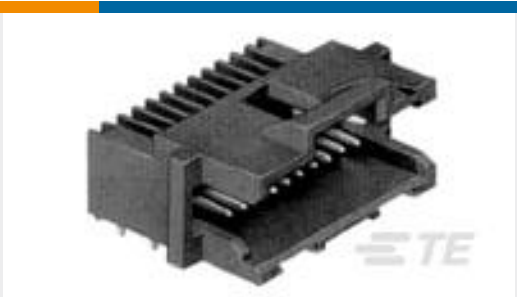
TE Part #1-338310-2 15POS.HD20 PLUG ASS'Y
