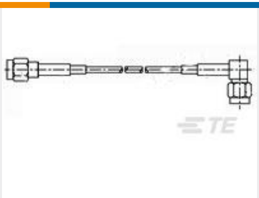
TE Part #1337810-1 50 OHM COAX SMA STR PLUG ELB P
